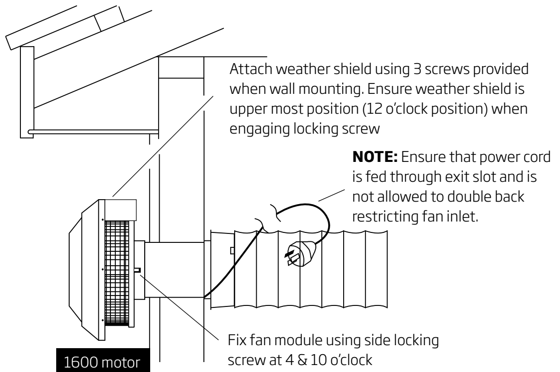
Figure 3 Wall Mount Option
