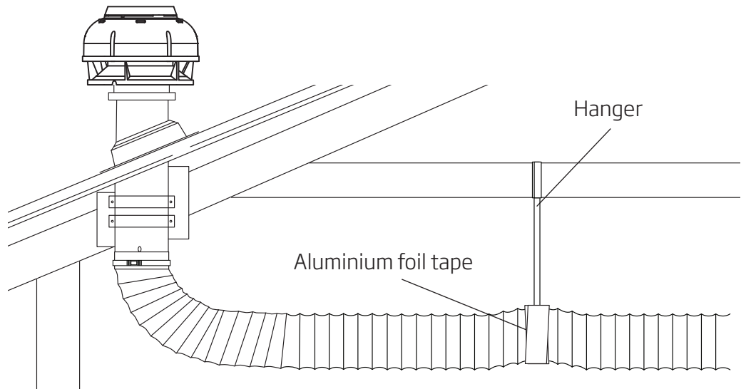
Figure 12: Securing SteelFlex™ Safety Duct
