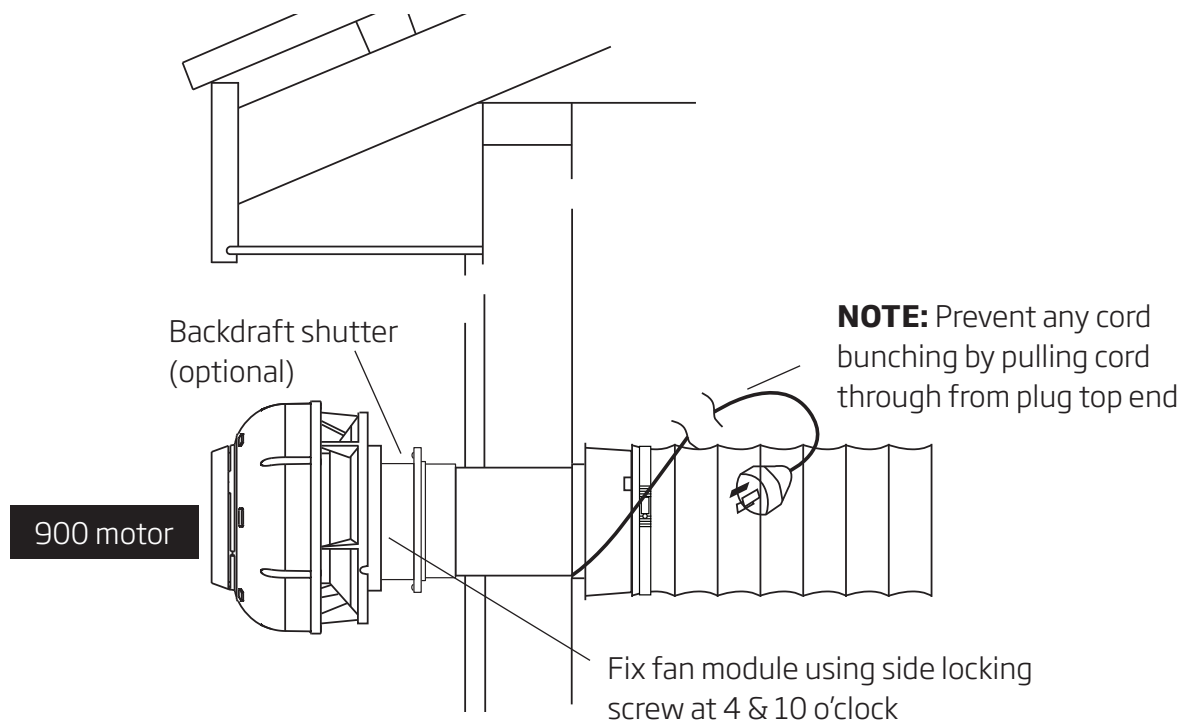
Figure 3: Wall mount option
