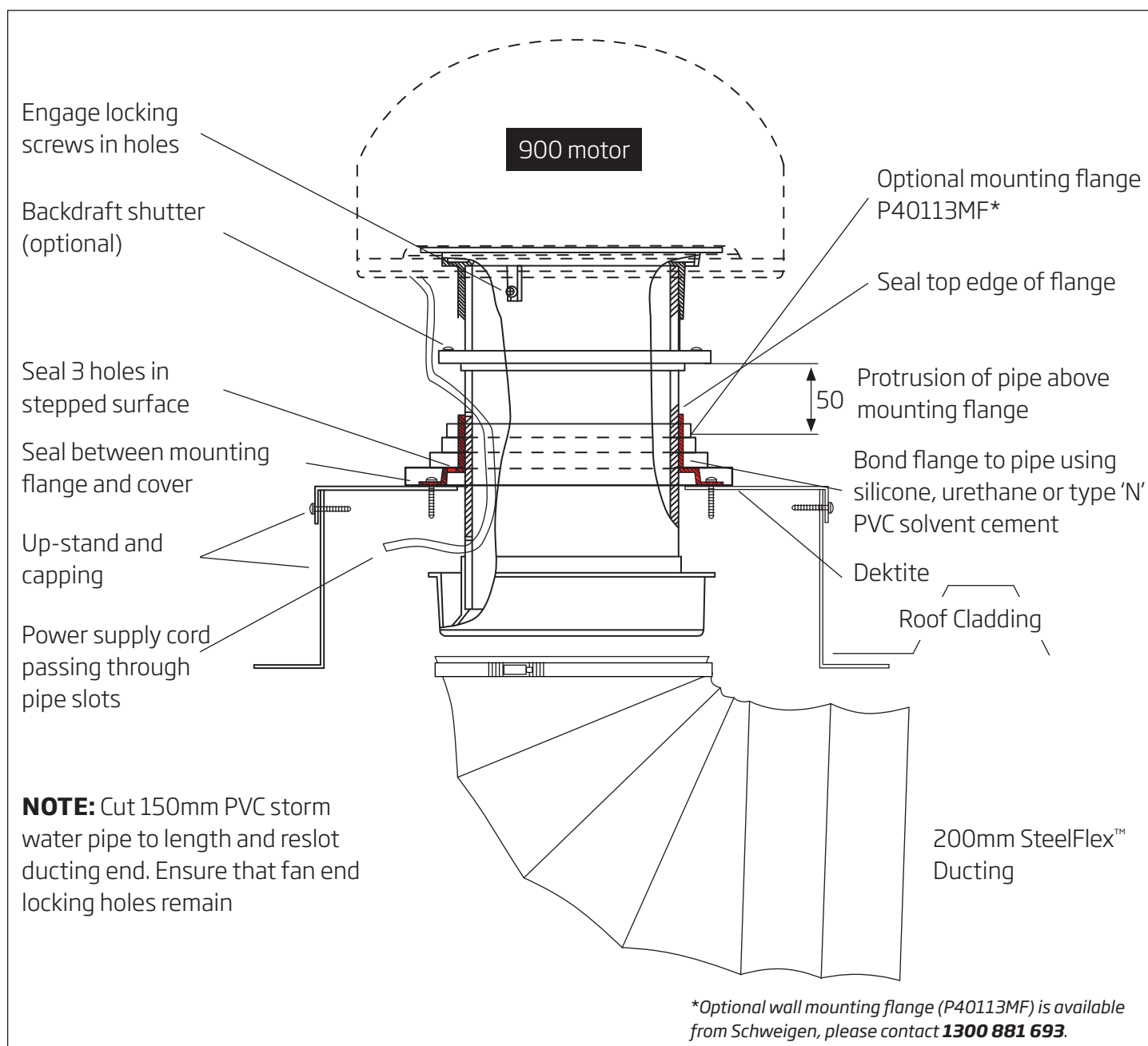
Figure 4: Flat roof installation
