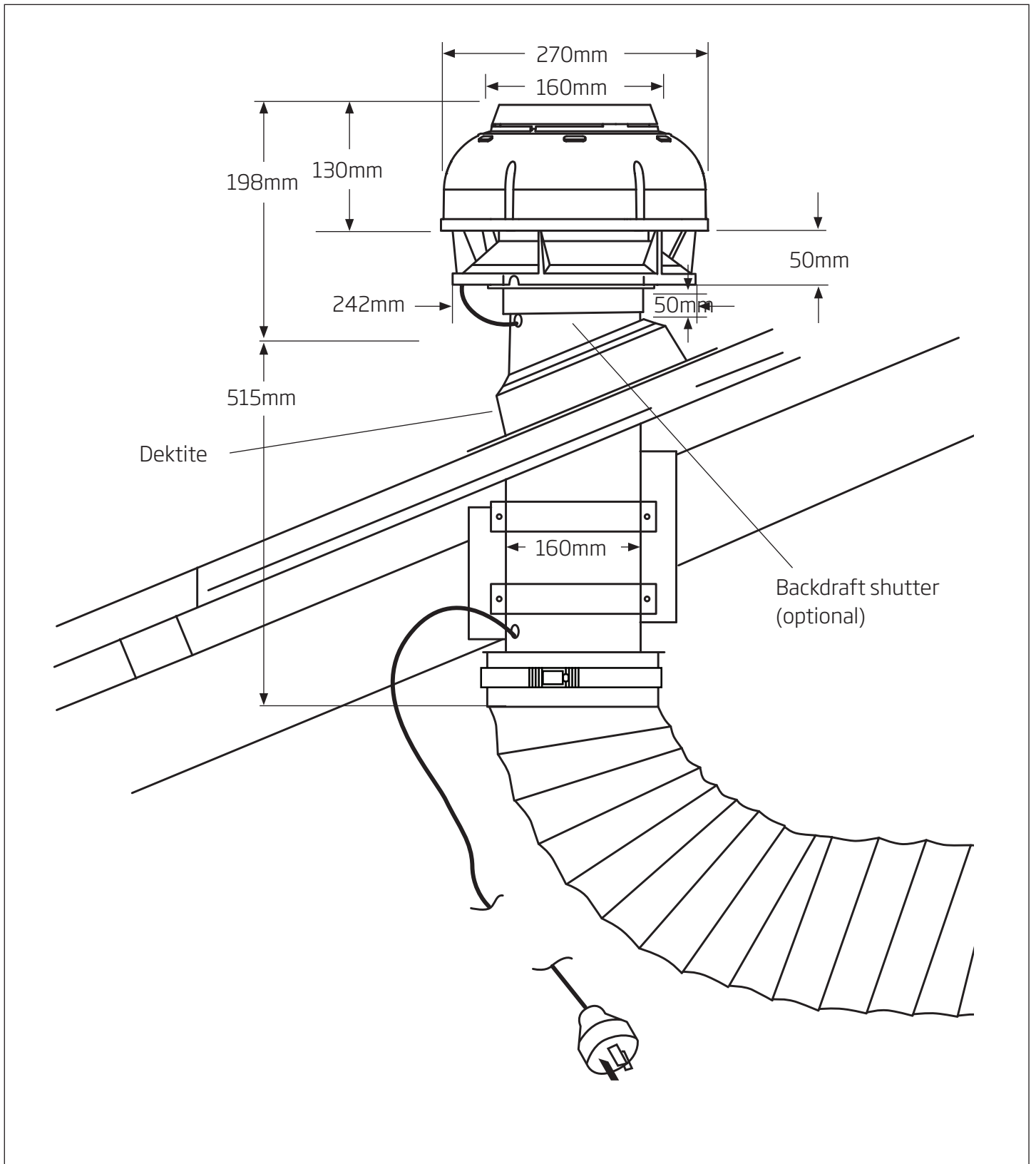
Figure 7: Measurements for Isodrive 900
