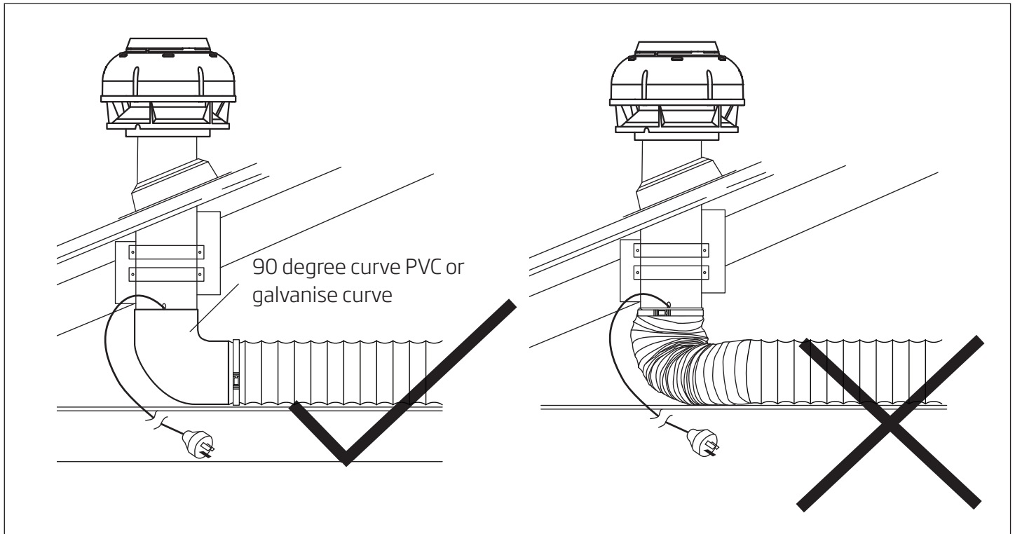
Figure 10: Shallow roof space
