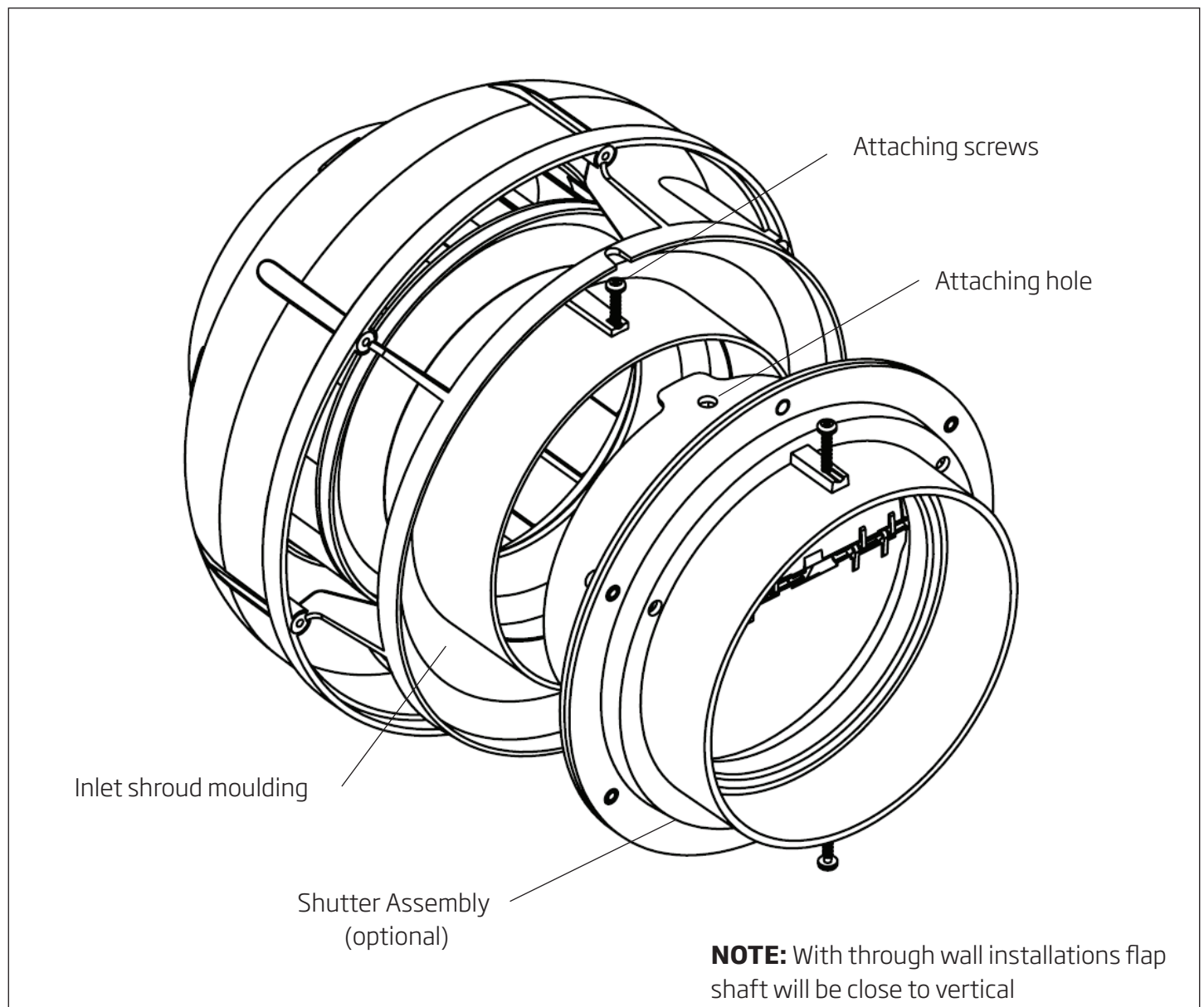
Figure 6: Shutter assembly
