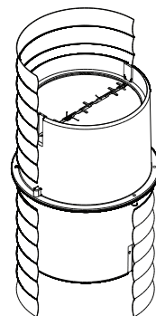
Back draught shutter in-line for 150mm ducting SCBDSSIL150MM
