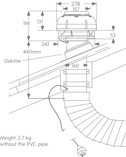
ST - IsoDrive 900 (900m 3 /hr)
