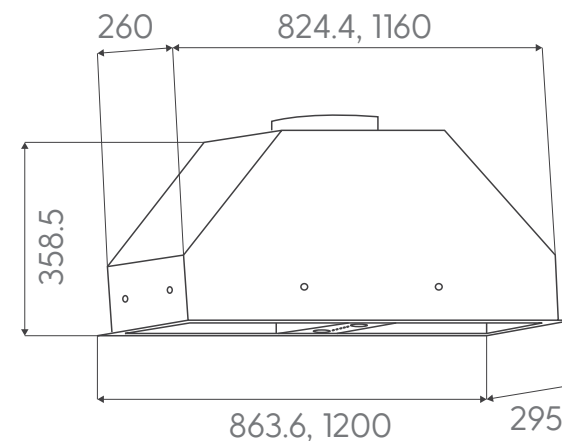
UM-9S and UM-12UMS
