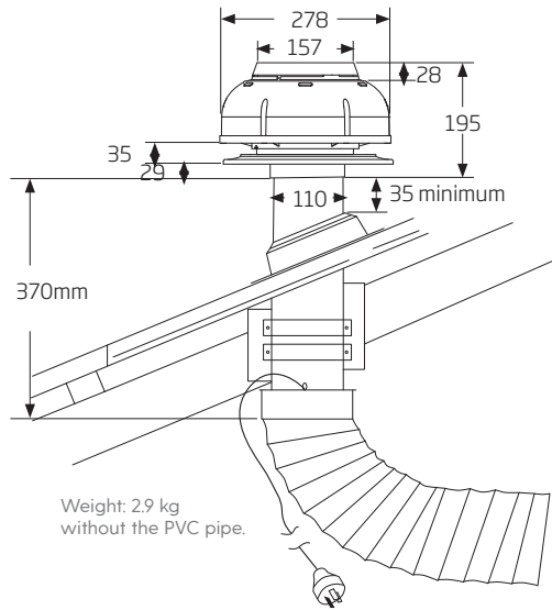
S1 - IsoDrive 650 (650m 3 /hr)
